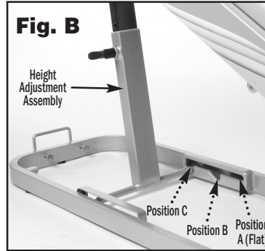
Fig. B Height Adjustment Assembly Position C Position B Position A (Flat)
